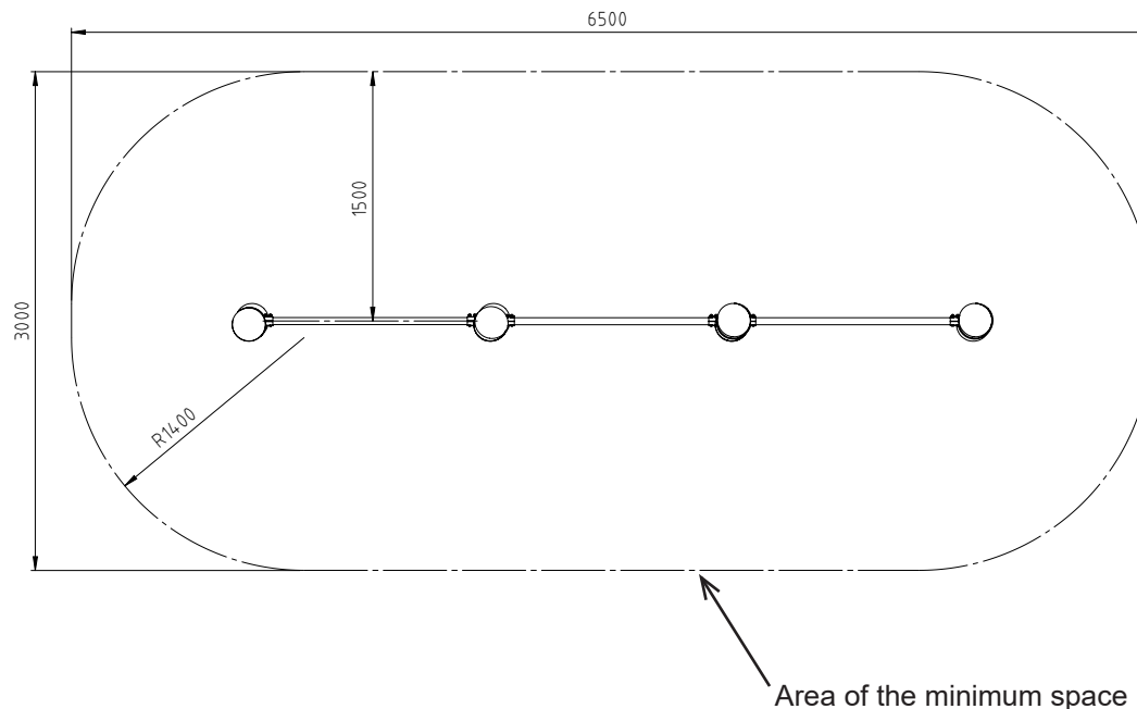
Diagram 4: Top view
